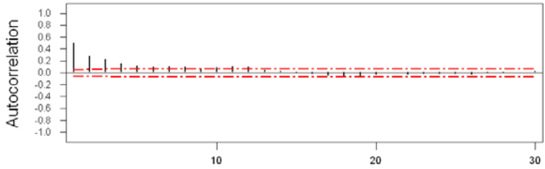
< Figure 3-3: The ACF plot of the detrended and deseasonalized observations >
