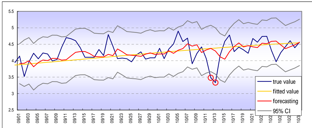
< Figure 5-10: Results of the prediction for X_{t+2} - Spectral Analysis >
