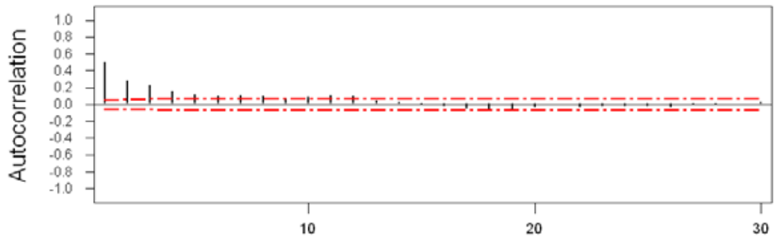
< Figure 3-8: The ACF plot of \varepsilon_t >
