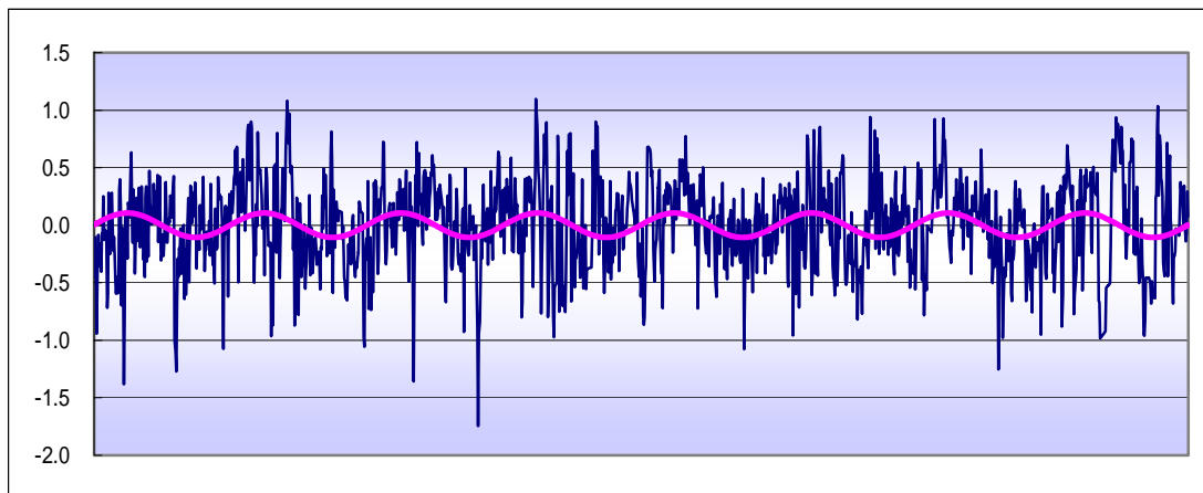
< Figure 3-7(b): The series \{\varepsilon_t\} with a fit >
