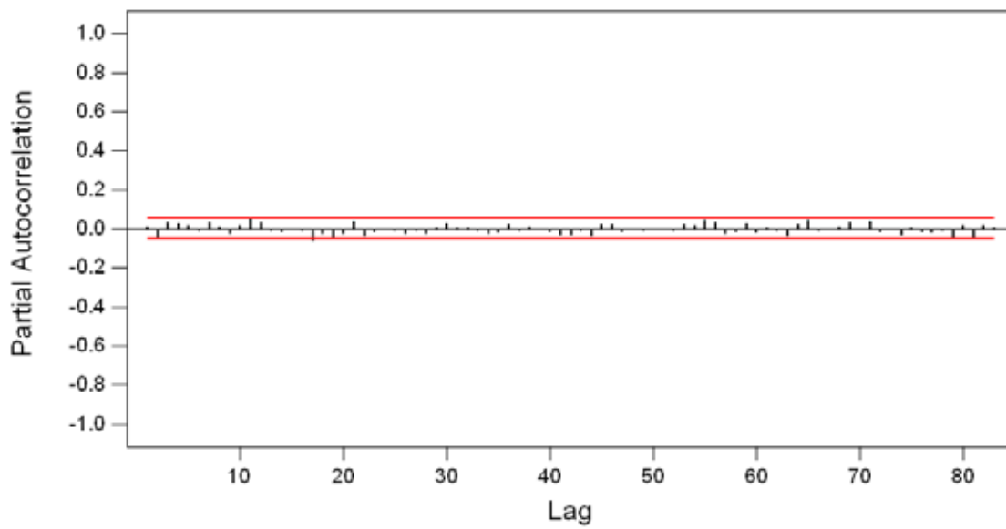
< Figure 4-7: The PACF plot of \xi_t >
