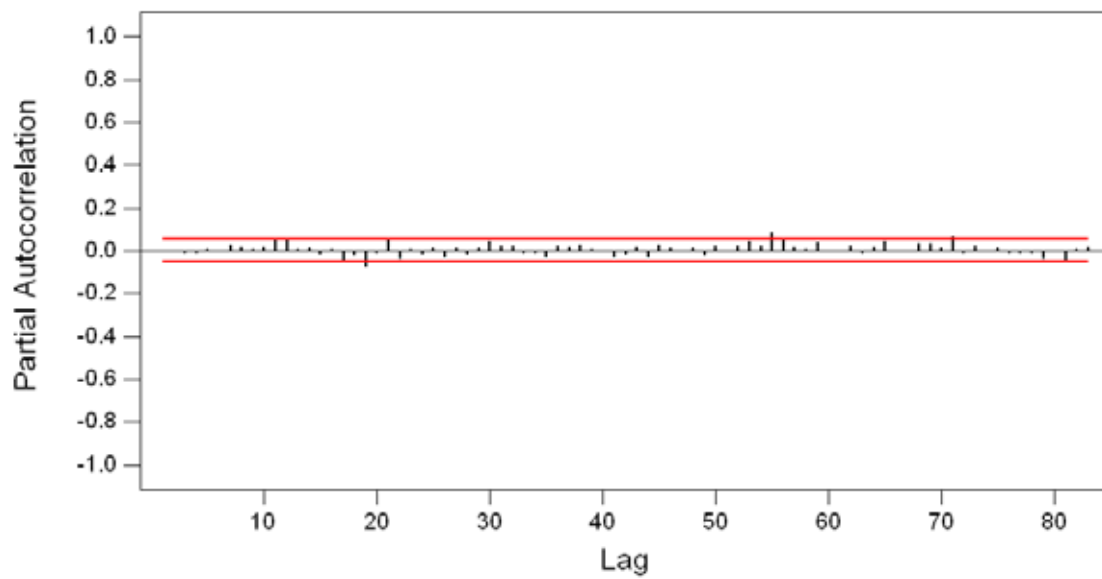
< Figure 3-6: The PACF plot of \eta_t >
