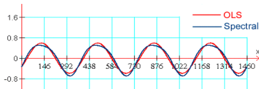
< Figure 5-8: The OLS fit and Spectral Analysis fit >
