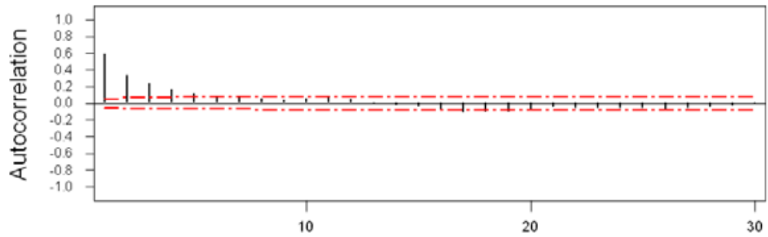
< Figure 4-4: The ACF plot of n_t >
