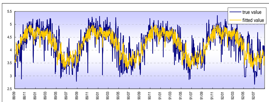
< Figure 5-1: True values VS Fitted values - The Small Trend Method >
